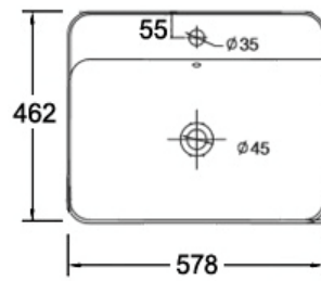
11479T-VC1-0 Semi Recess Basin 578mm Taphole - 1
