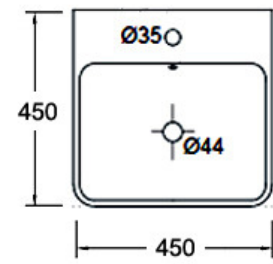
24985K-1-0 Wall Basin 450mm Taphole - 1
