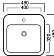
Y0M8 Semi Recess Basin 480mm
