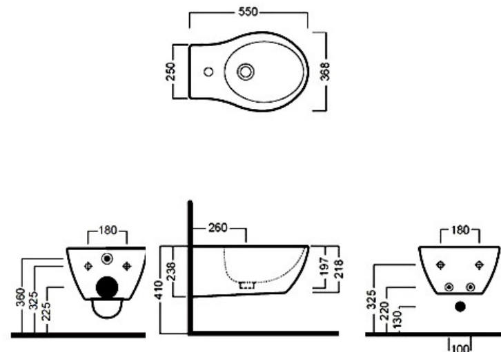
Y0U0 Wall Hung Bidet Taphole - 1
