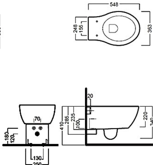
Y0U2+YXWW Wall Hung WC Soft Close Seat
