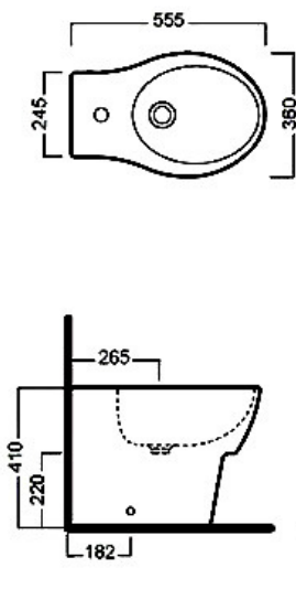
Y0QW Wall Faced Bidet Taphole - 1
