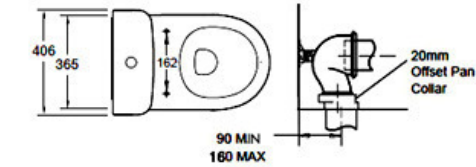
21001A-0 Back to Wall Suite Soft Close Seat
