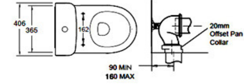
77303A-0 Wall Faced Suite Soft Close Seat
