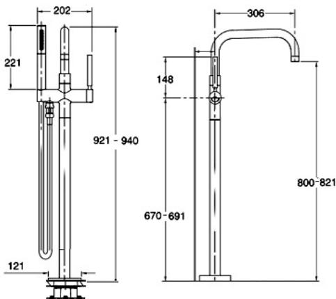
10129A-B4-CP+97905T-DR-NA Freestanding Bath Spout Chrome
