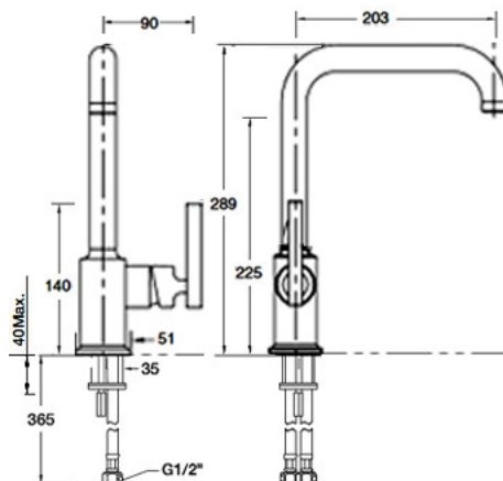
14597A-4-CP Sink/Laundry Mixer Chrome
